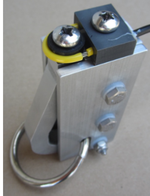
Pelican Hook Mount (REL-124) provides 5:1 mechanical advantage, holding up to 750-lb static weight
