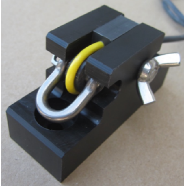
Burnwire Mount (REL-158) provides a secure mount to a lander frame
